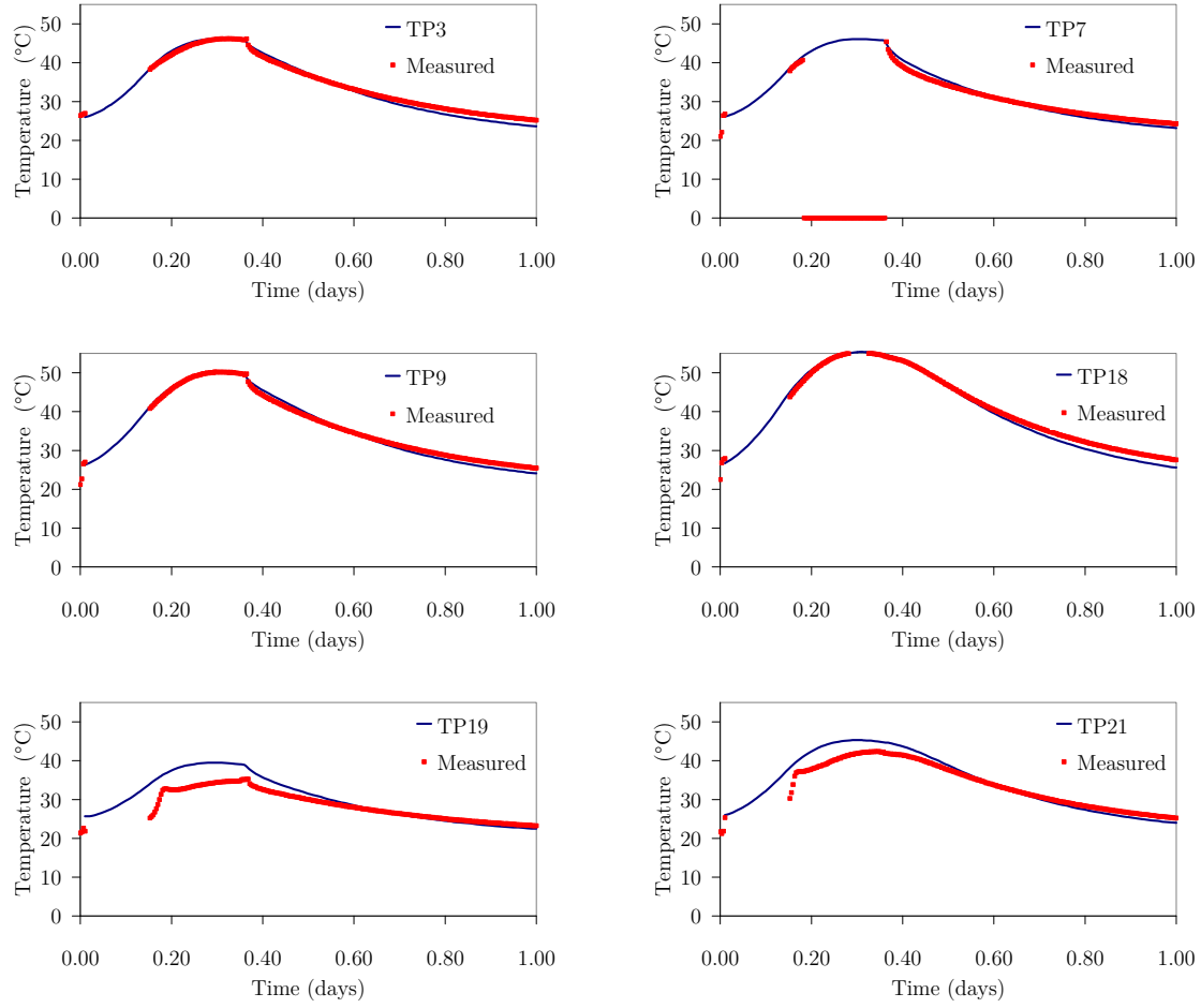
Figure 2.31: Comparison of temperatures: experimental (thermocouples) versus numerical results
