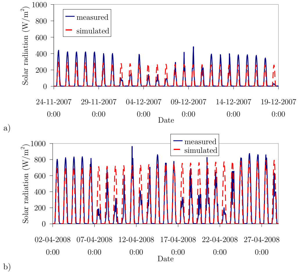
Figure 6.59: Comparison of measured and predicted values of solar radiation on a horizontal surface: a) November/December 2007 ; b) April 2008
