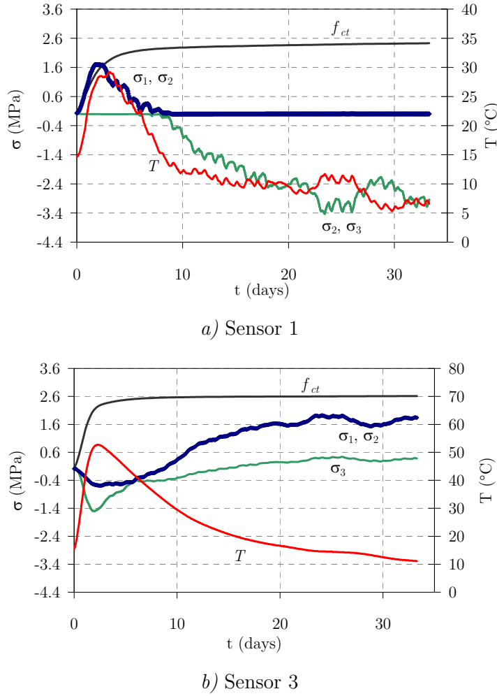
Figure 6.16: Evolution of principal stresses and temperatures close to sensors 1 and 3
