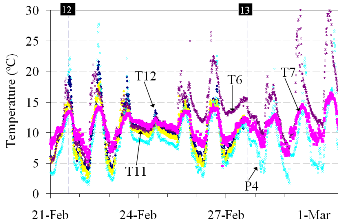
Figure 6.42: Environmental temperature measurements – from 21 st February until 2 nd March
