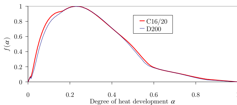
Figure 6.56: Normalized heat generation function f(\alpha)
