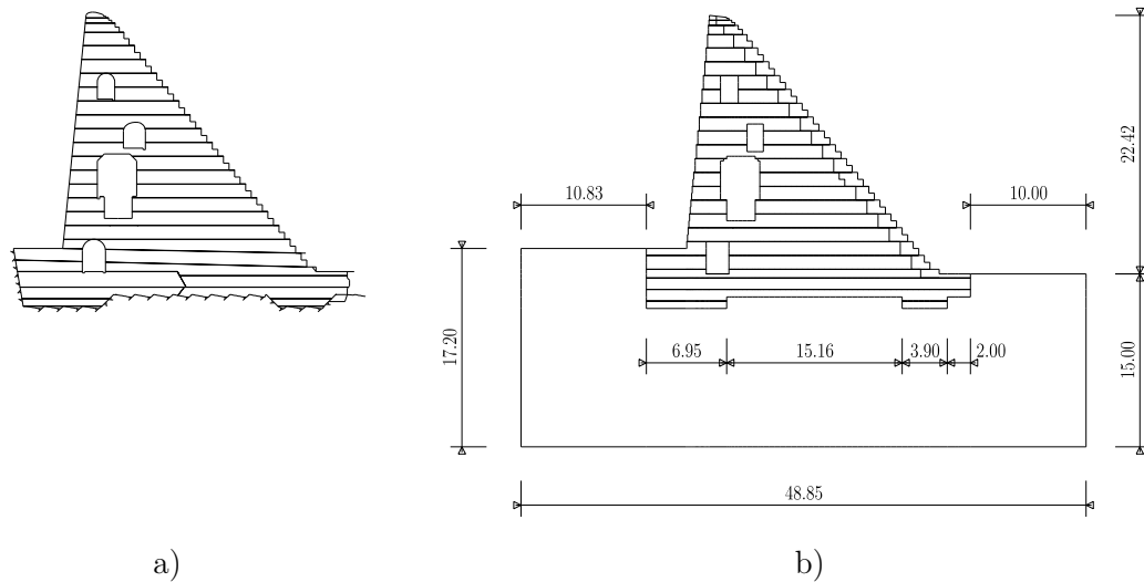
Figure 6.54: a) Real geometry of the dam in block 9; b) Geometry adopted for the FE model (units: m)
