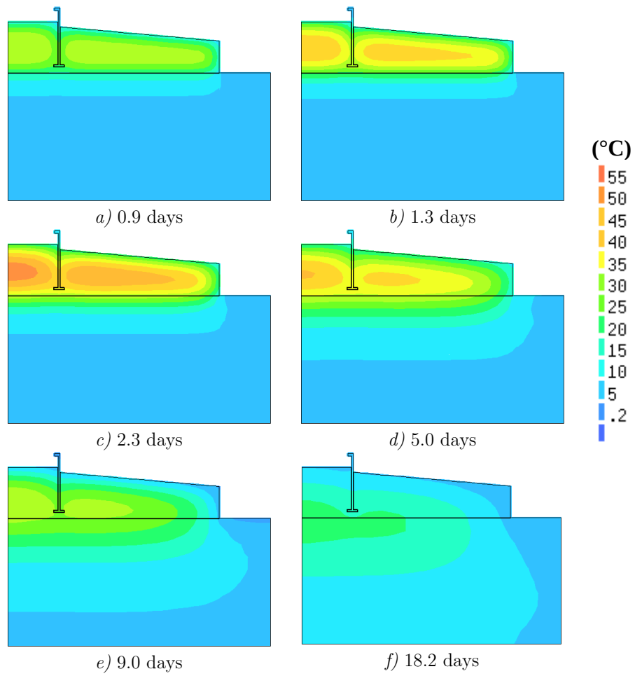
Figure 6.11: Evolution of calculated temperatures
