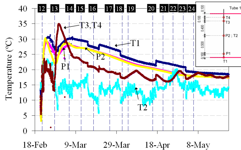
Figure 6.37: Temperature measurements along tube 1 (sensors located in Phase 12)
