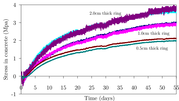
Figure 5.26: Tensile stresses in concrete computed from the steel strains
