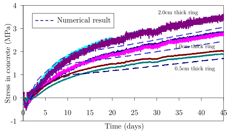
Figure 5.30: Stresses in concrete: numerical versus experimental
