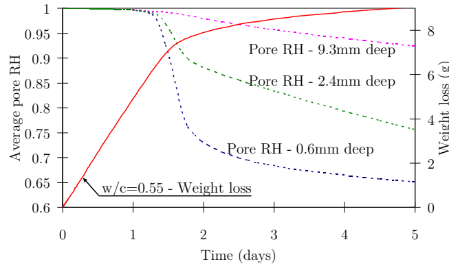
Figure 4.29: Evolution of pore RH and weight loss for T=20^{\circ}\text{C} and \text{RH}=60\% - numerical simulation
