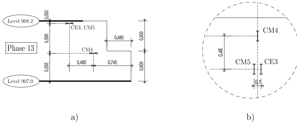
Figure 6.35: Schematic representation of strain gages near the downstream surface: a) elevation; b) plan (units: m)
