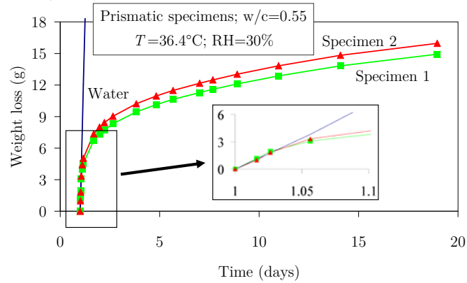
Figure 4.23: Weight losses: evaporative cooling tests ( w/c=0.55 )
