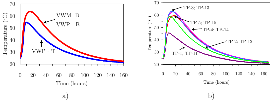
Figure 5.7: Temperatures measured by: a) the vibrating wire strain gages; b) the thermocouples on the lateral boundaries
