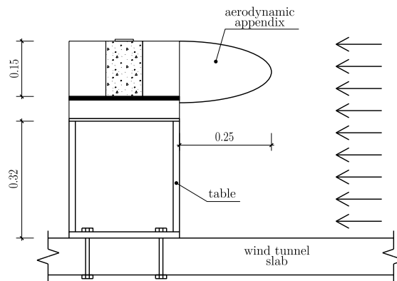
Figure 2.55: Setup of specimen in the wind tunnel (units: m)
