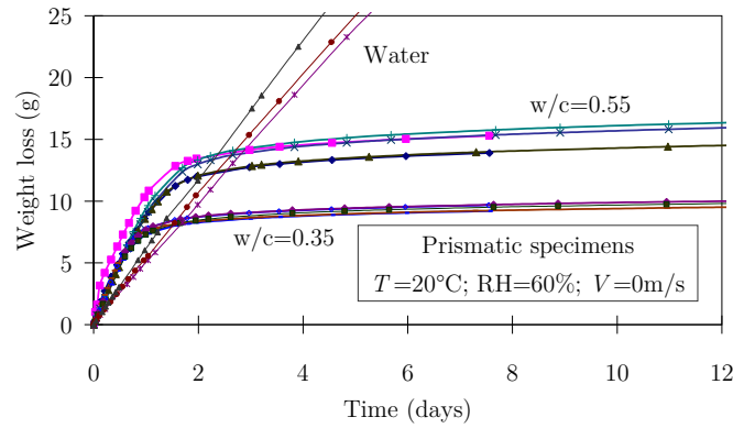
Figure 4.13: Weight losses for wind speed V=0\text{m/s}
