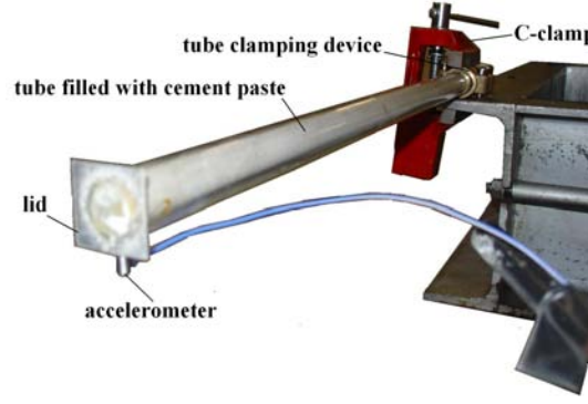
Figure 5.48: Photo of experimental setup
