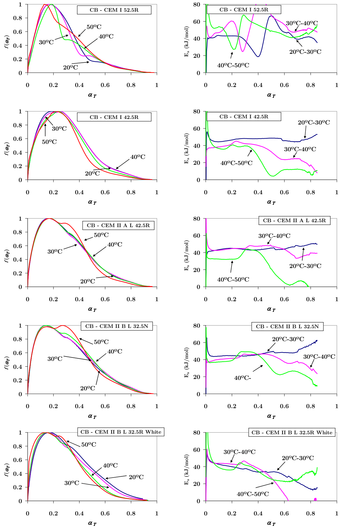
Figure 2.17: Company B cements: a) f(\alpha_T) ; b) E_a
