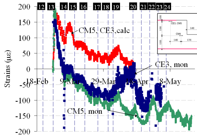
Figure 6.80: Monitored and calculated strains for CM5, CE3
