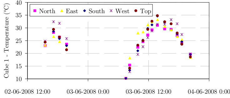
Figure 2.45: IR Temperature measurement results – Cube 1
