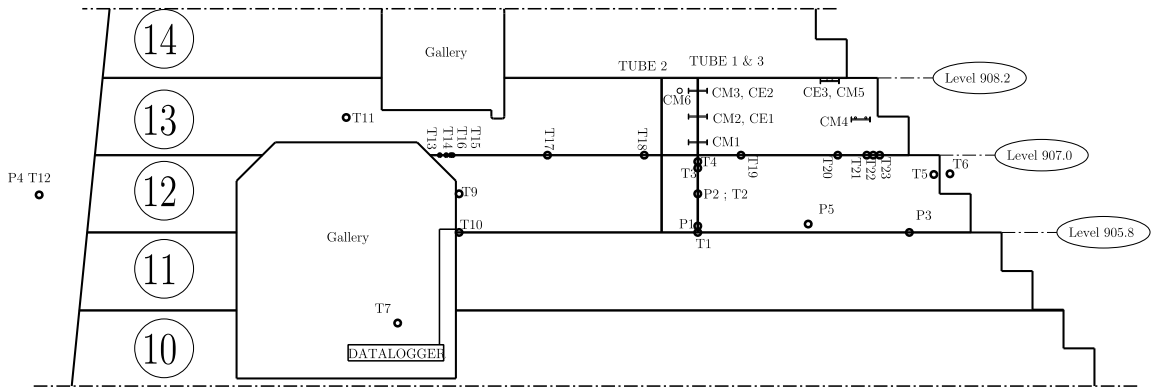
Figure 6.26: Elevation of phases 12 and 13 – location of temperature and strain sensors
