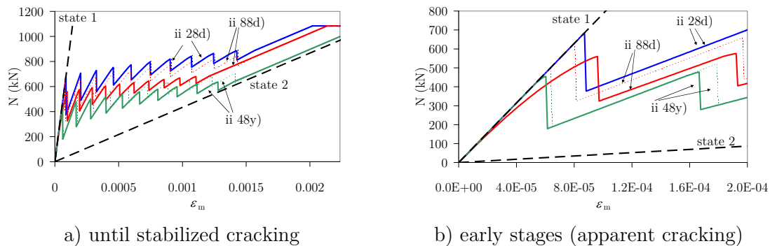
Figure 5.75: N - \varepsilon_m relationships for imposed axial deformations at different ages for the model considering differential drying shrinkage (continuous lines) versus model considering uniform drying shrinkage (dashed lines)
