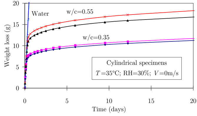
Figure 4.10: Weight losses for environment with T=35^{\circ}\text{C} , \text{RH}=30\%
