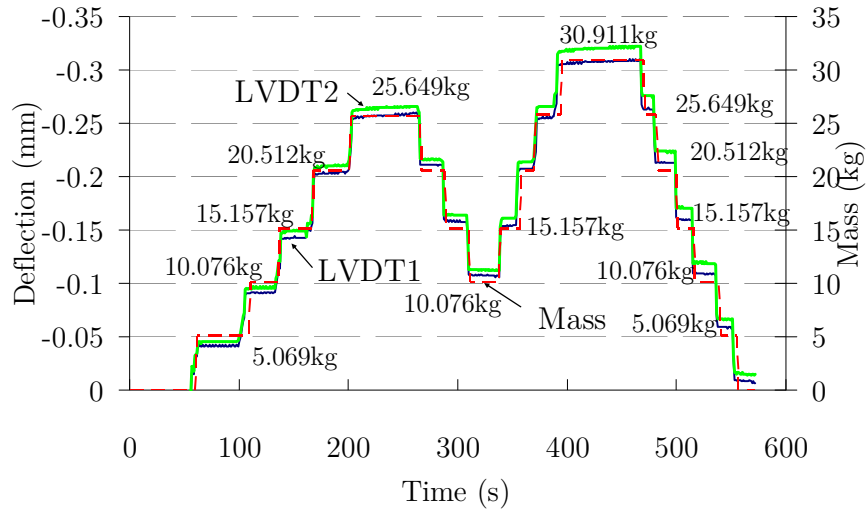
Figure 5.41: Mid-span masses and deflections during the static test
