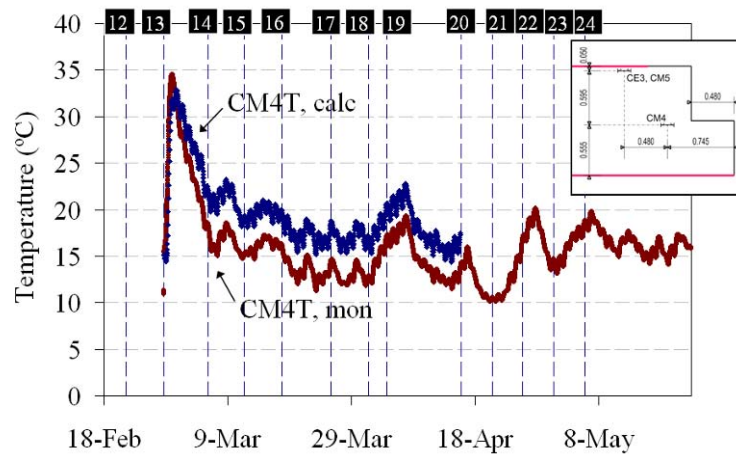
Figure 6.72: Monitored and calculated temperatures for CM4T
