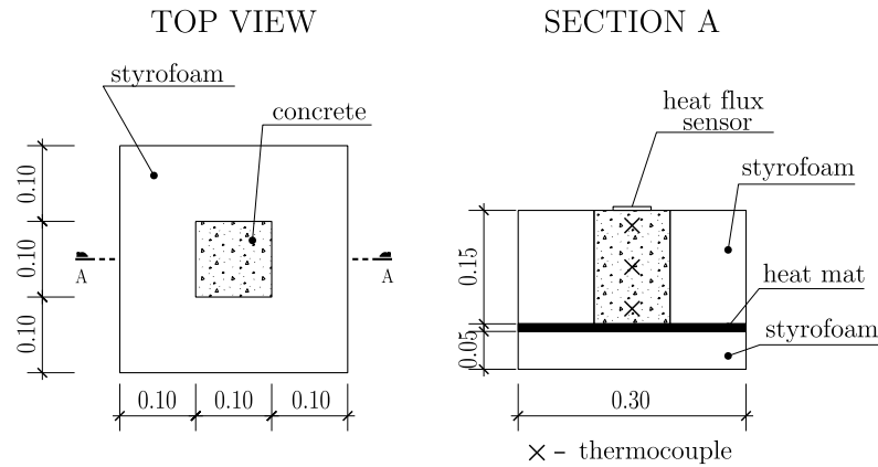
Figure 2.54: System for heat generation and temperature measurement in the concrete specimen (units: m)
