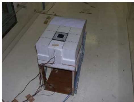
Figure 2.56: Photo of experimental setup inside the wind tunnel (view from downstream)
