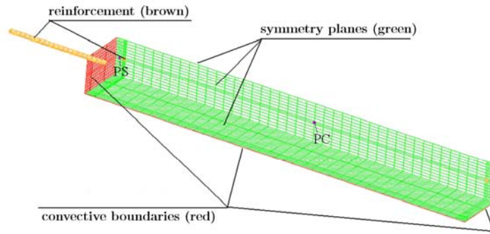
Figure 2.38: FE mesh for the RC element
