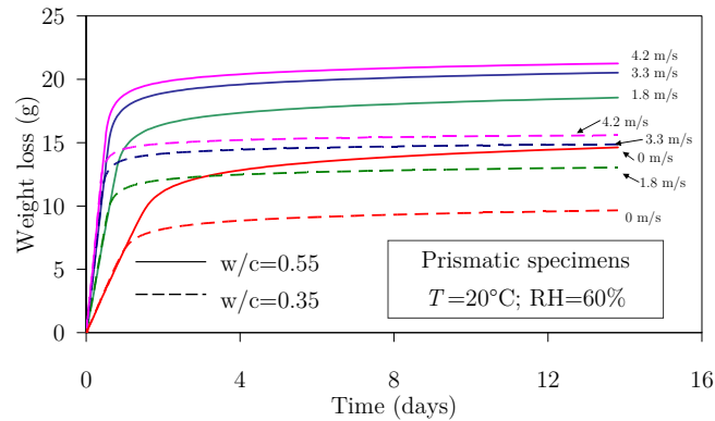
Figure 4.35: Weight losses under variable wind speed - numerical simulations
