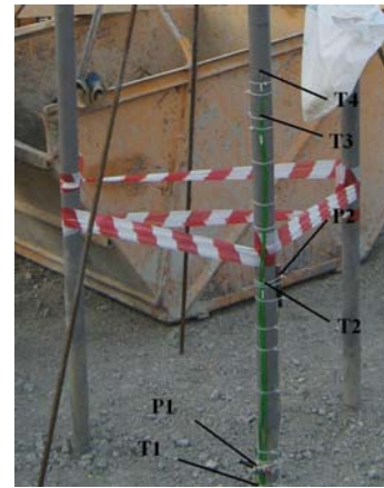
Figure 6.28: Placement of temperature sensors along tube 1 (phase 12): a) scheme; b) photo
