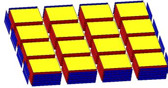
Figure 4.54: Adopted FE mesh for specimens
