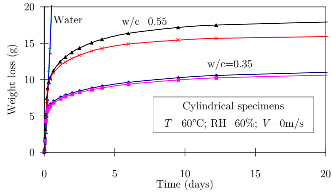
Figure 4.11: Weight losses for environment with T=60^{\circ}\text{C} , \text{RH}=60\%
