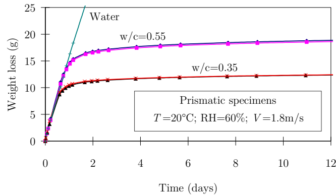
Figure 4.14: Weight losses for wind speed V=1.8\text{m/s}
