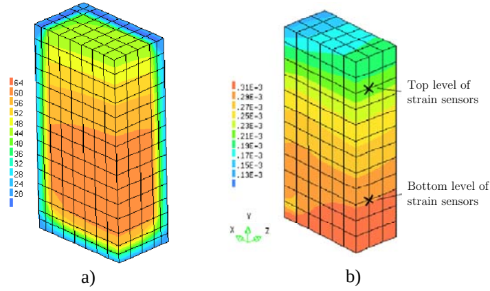
Figure 5.12: Numerical results for t=15.8\text{h} : a) temperatures ( ^{\circ}\text{C} ); b) total strains \epsilon_x
