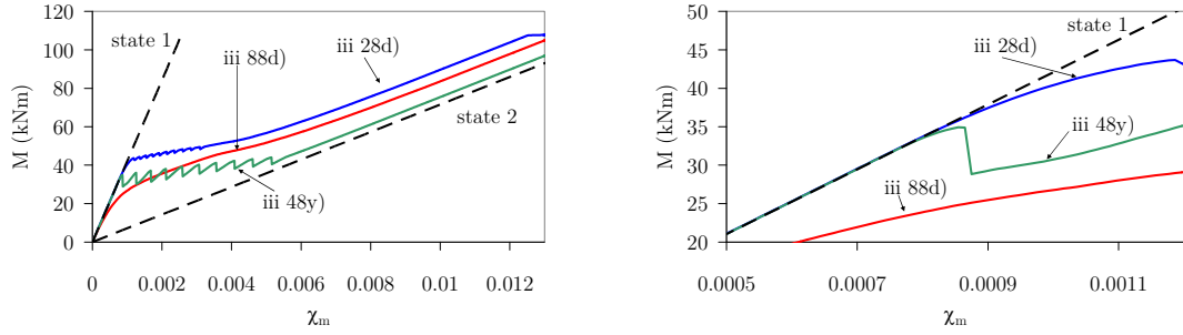
a) representation until stabilized cracking b) early stages (apparent cracking) Figure 5.76: M-\chi_m relationship for imposed curvature tests at the different ages of 28 days, 88 days and 48 years
